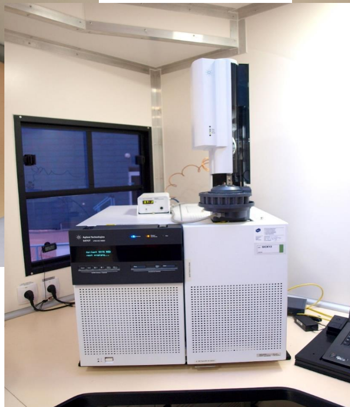
Gas chromatography with a mass spectrometer
